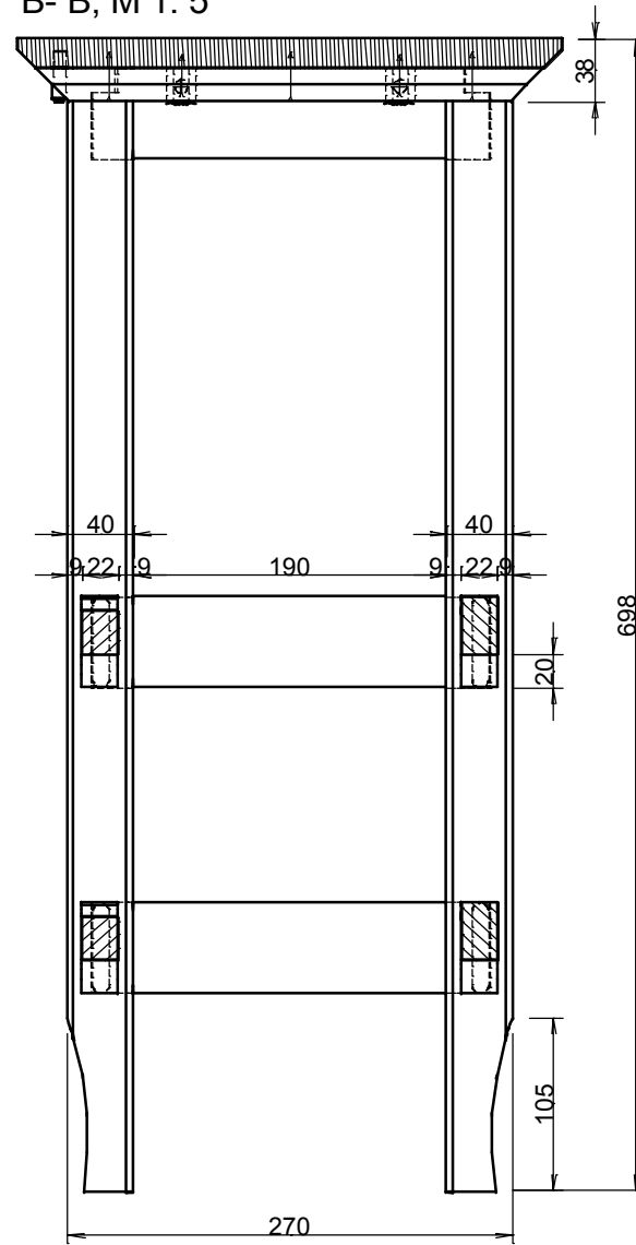
B-B, M 1: 5
