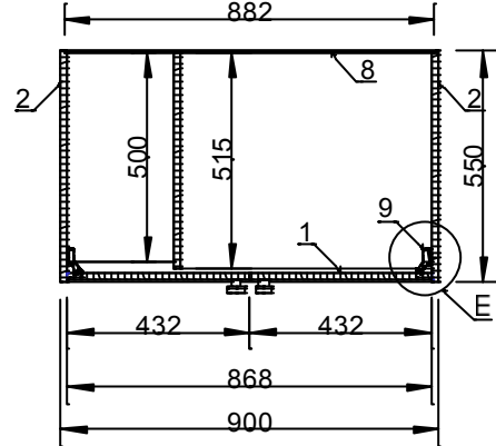
E-E, M 1:20
